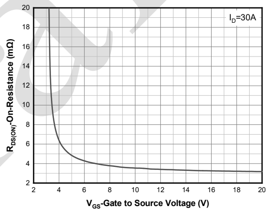
On-Resistance vs. Gate-to-Source Voltage (4)
