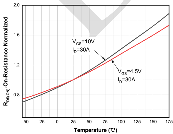
On-Resistance vs. Junction Temperature (4)
