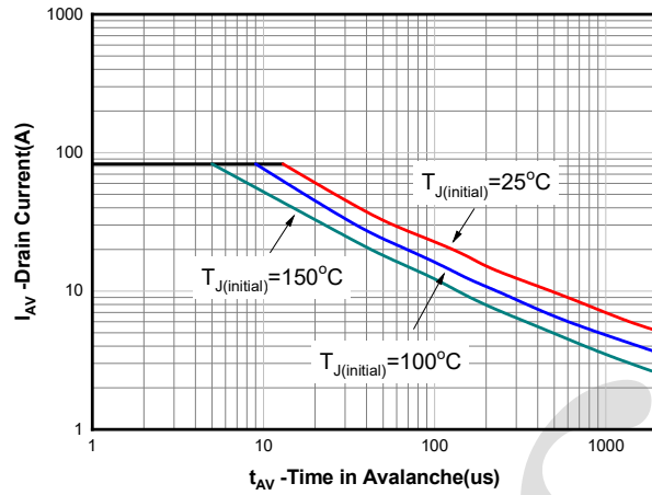
Avalanche characteristics
