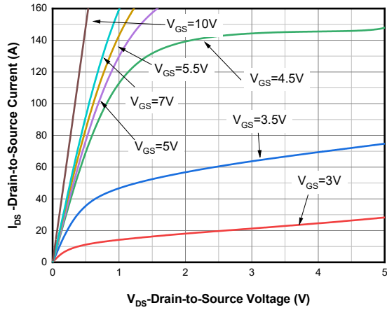
Output Characteristics (4)
