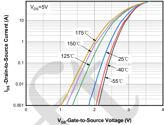
Transfer Characteristics (4)
