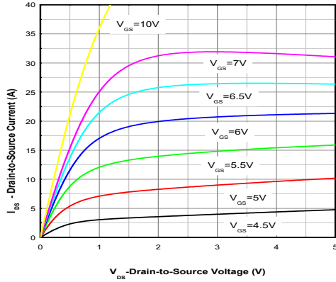
Output Characteristics (4)
