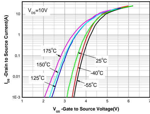
Transfer Characteristics (4)
