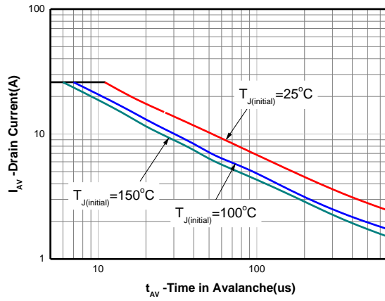
Avalanche characteristics
